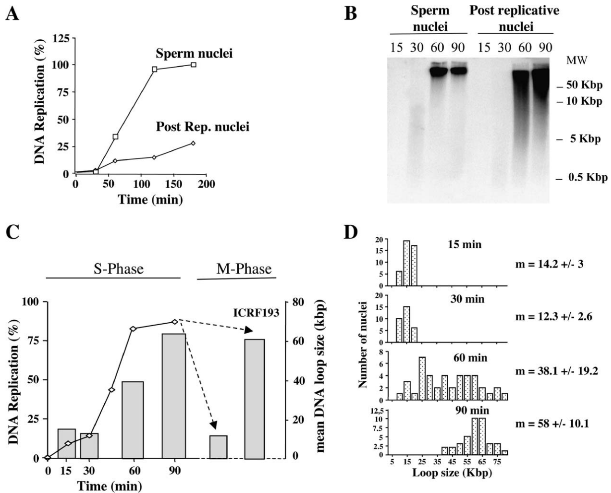
Figure 7. Mitotic Remodeling of Chromatin Loop Domains Occurs in S and M Phases
