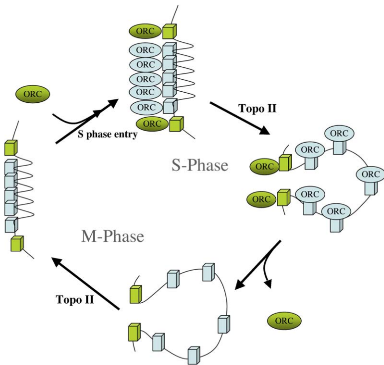
Figure 8. Cell-Cycle Remodeling of Chromatin Organization in the Early Xenopus Embryo
