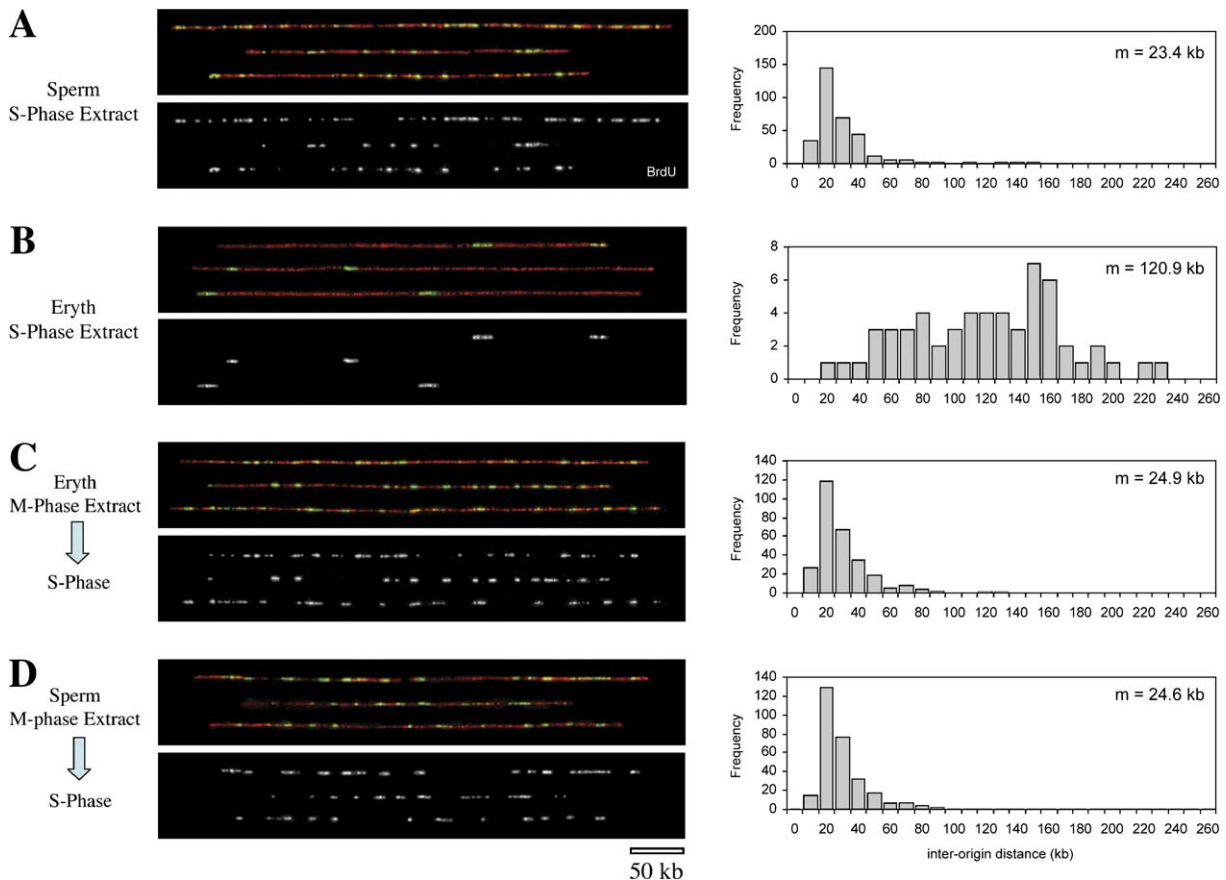
Figure 2. Single-Molecule Analysis of the Interorigin Spacing by Molecular Combing
