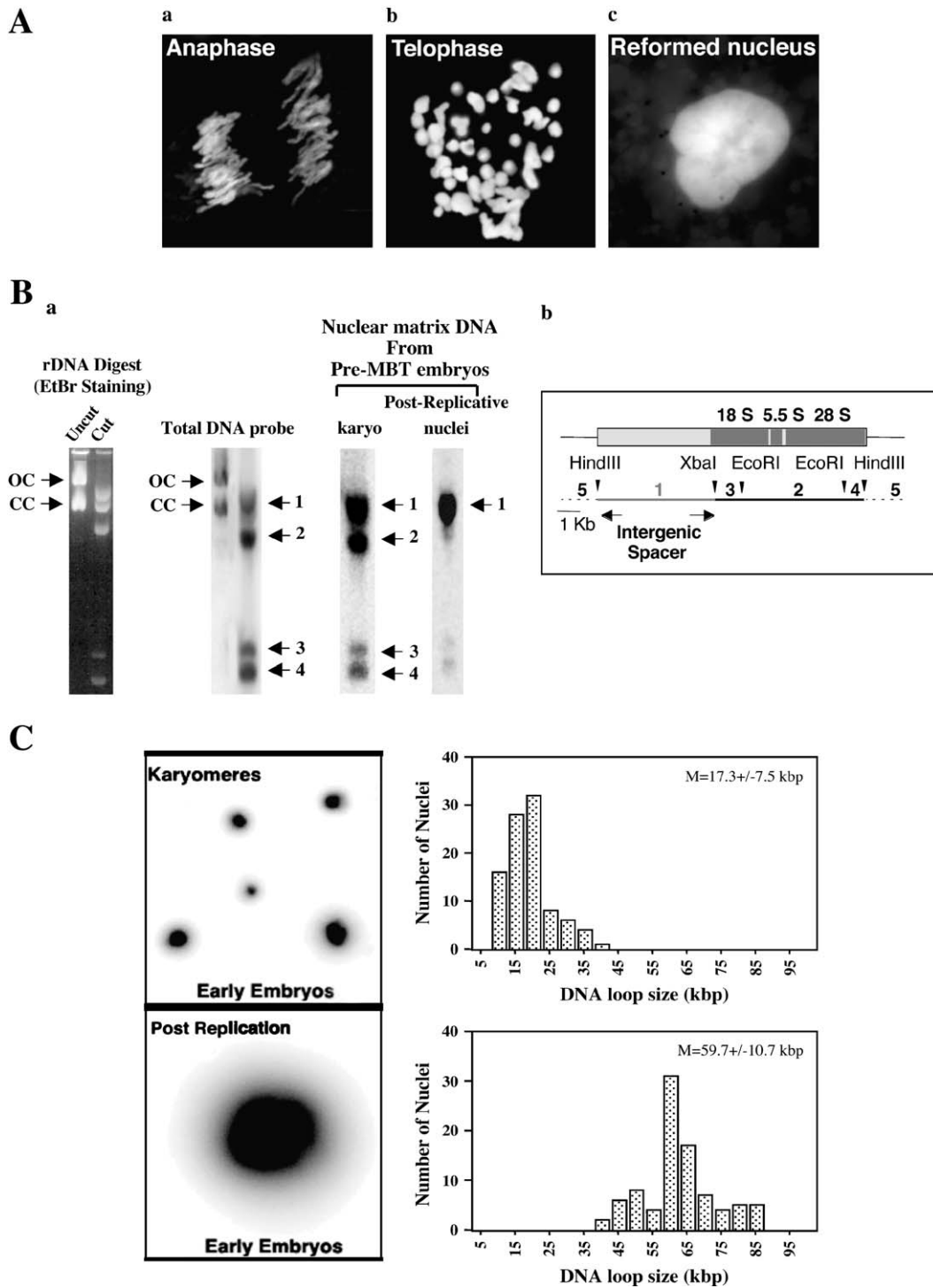
Figure 6. Cell-Cycle Remodeling of Chromatin Organization in Early Xenopus Embryos
