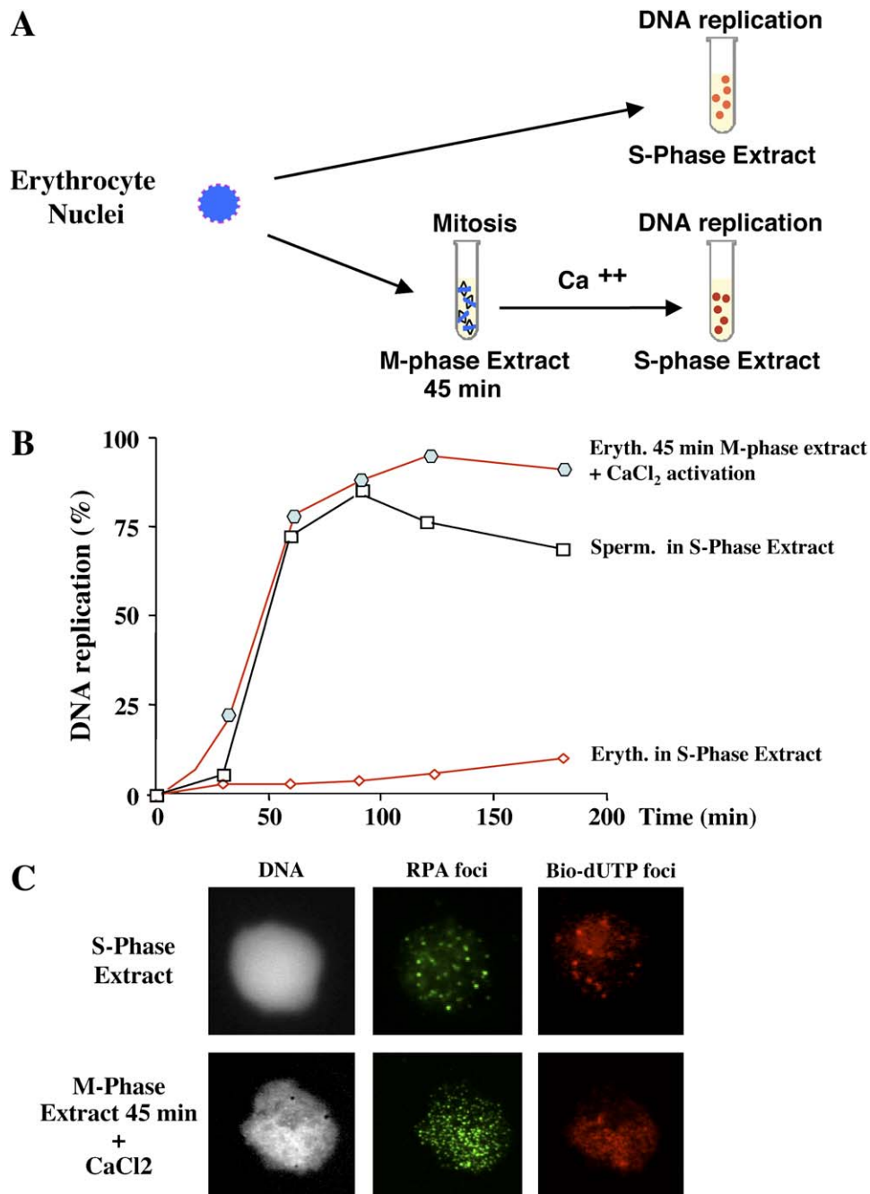
Figure 1. Exposure to M Phase Conditions Makes Erythrocyte Nuclei Fully Competent for DNA Replication
