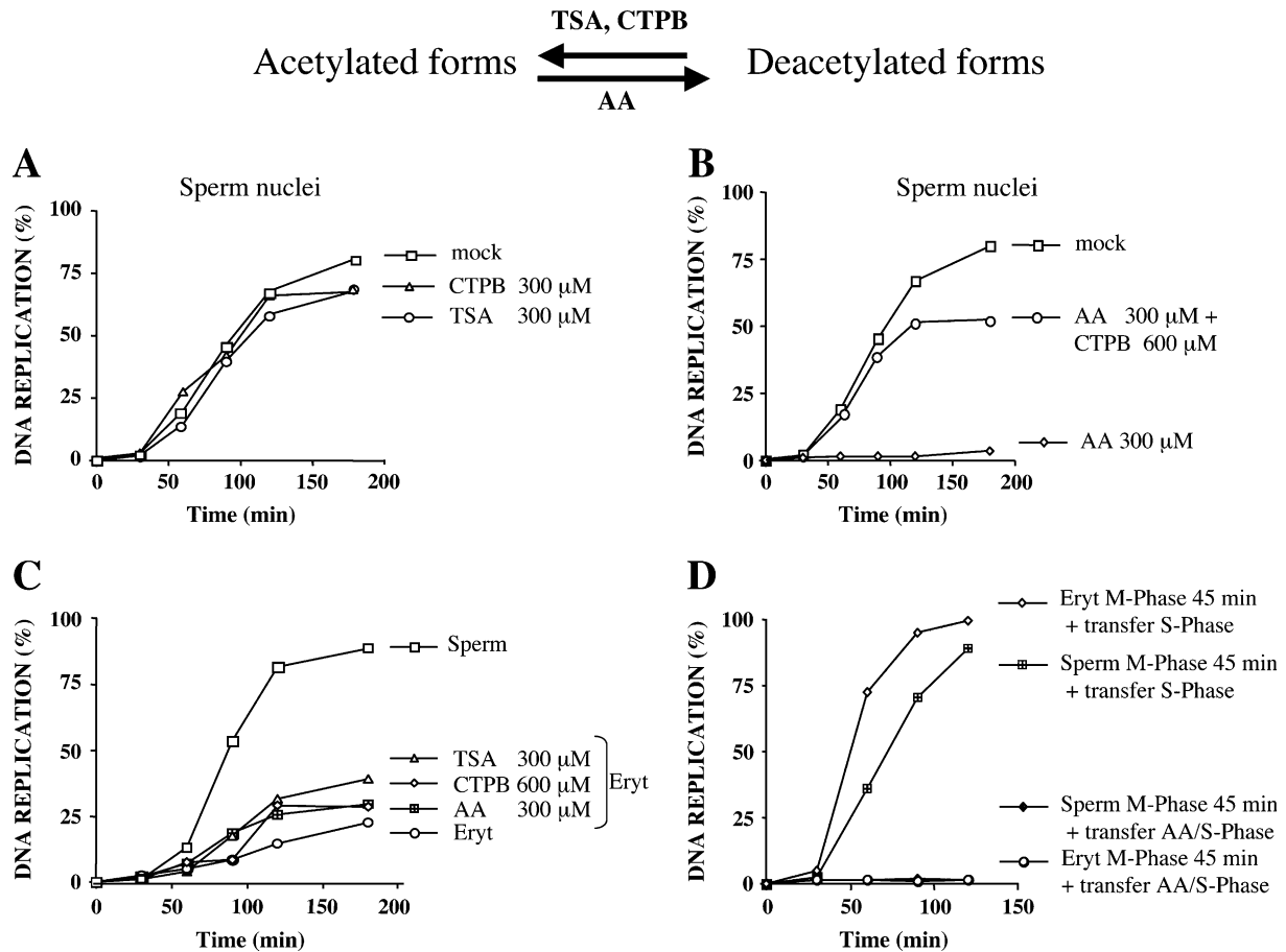
Figure 3. Histone Acetylation Does Not Induce Erythrocyte Nuclei Remodeling
