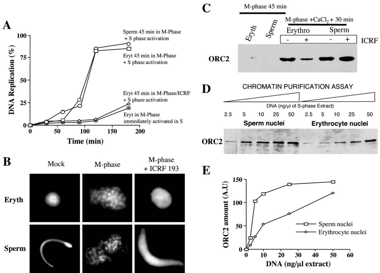
Figure 5. ORC Binding and DNA Replication Efficiency Depend on the Chromatin Context and Topoisomerase II Activity (A) Erythrocyte chromatin was incubated either in M phase extract and immediately driven into S phase by Ca 2+ or in M phase extract for 45 min before induction into S phase by Ca 2+ in the absence or presence of ICRF 193. Control sperm chromatin in M phase extracts induced to enter S phase by calcium is shown. The amount of nuclei was 1000 nuclei/μl egg extract for sperm nuclei and 500 nuclei/μl egg extract for erythrocyte nuclei, to keep the chromatin concentration constant. (B) Demembrated sperm nuclei or erythrocyte nuclei were incubated in a mitotic egg extract in the presence or absence of 50 μg/ml of the topoisomerase II inhibitor ICRF 193. DNA was stained with Hoechst dye for chromosome formation analysis. (C) Chromatin was purified and proteins were analyzed by SDS gel electrophoresis as described in Experimental Procedures . Sperm nuclei (1000 nuclei/μl egg extract) or erythrocyte nuclei (500 nuclei/μl egg extract) were incubated in a mitotic egg extract induced to enter S phase with calcium in the presence or absence of ICRF 193. Chromatin was purified 30 min after calcium activation and analyzed by immunoblot with a Xenopus anti-ORC2 antibody. (D) Erythrocyte nuclei and sperm nuclei were incubated for 30 min in S phase extract at various DNA concentrations. Chromatin was purified and analyzed by 10% SDS-PAGE. (E) Quantitation from the immunoblot.
